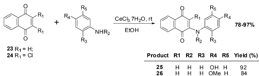
Scheme 4 Synthesis of phenylaminonaphthoquinones.
