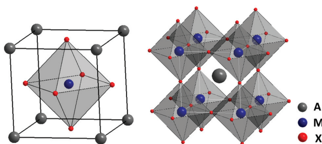
Fig. 1 Crystal structure of cubic perovskite of general formula ABX_3 .
