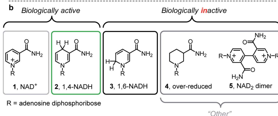
Fig. 2 Cofactor compositions after H 2 -driven NAD + reduction by different chemo/C catalysts. a . Values were calculated using a combination of quantitative 1 H NMR spectroscopy and UV-visible spectroscopy at three time points ( t_1 = 30 min, t_2 = 2 h, t_3 = 17 h). At 17 h, 5–8% relative standard deviation was determined from reactions performed in triplicate using 3 wt% Pd/C (Fig. S1, ESI†). Reaction conditions: 2 mL of 5 mM NAD + in Tris–HCl (50 mM, pH 8.0) was stirred with 0.32 mg commercial chemo/C under a steady flow of H 2 (1 bar) at room temperature. “Blank” experiments were run as a control in the absence of catalyst, and our previous report showed that carbon black (BP2000) does not catalyse H 2 -driven NAD + reduction. 14 Further details in ESI (S1.5.1†). (b) Simplified structures of biologically active and inactive nicotinamide cofactors.
