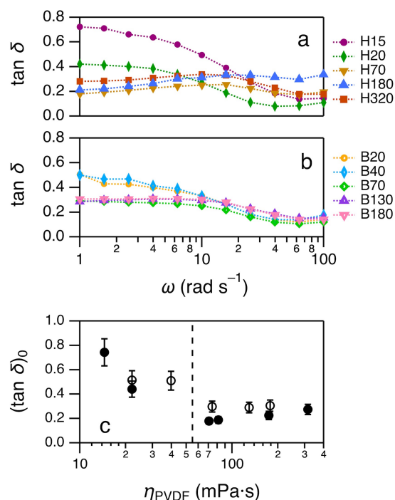
Fig. 3 Viscoelastic characterisation of cathode slurries comprising NMC811/CB/PVDF in the ratio 95:5:5 and 43 wt% solid loading in solutions of PVDF/NMP with varying viscosities. a) Loss tangent frequency sweeps for slurries comprising homopolymer binders Hxx and b) blended binders, where xx denotes the binder solution viscosity in \text{mPa}\cdot\text{s} . Dotted lines are a guide for the eye. c) Zero-frequency extrapolations of the loss tangent for slurries comprising homopolymers (●) and binder blends (○). The dotted line approximates the threshold viscosity above which \tan \delta does not vary.
