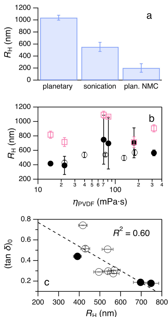
Fig. 6 DLS measurements of the hydrodynamic radius of carbon black particles. a) CB is dispersed in pure NMP using different mixing conditions: planetary mixing, sonication, and dry mixing with NMC followed by planetary mixing. b) CB was recovered from cathode slurries comprising NMC/CB/PVDF (90:5:5 by weight) with a solid loading of 43.1 wt%. The binder solution comprises either homopolymer PVDF (●) or a blend (○). The particle sizes of analogous dispersions of CB in PVDF/NMP solutions (without NMC) are shown for comparison (□). Error bars denote the half-width of the particle size distribution. c) Correlation between the viscoelasticity of slurries and the size of carbon black particles. The solid line shows a linear regression with R^2 = 0.60 .
