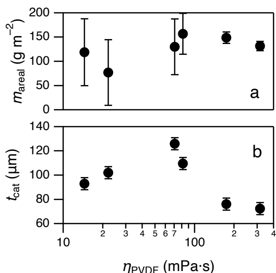
Fig. 8 Properties of formed cathodes of NMC811/CB/PVDF (95:5 w/w) across a series of different PVDF/NMP solution viscosities, \eta_{\text{PVDF}} . a) Areal mass loading, m_{\text{areal}} , of the composite cathodes and b) thicknesses of cathodes produced using a draw down velocity of 5.8 mm s -1 and a gap height of 285 μm. c) Porosity of cathodes produced under varying processing conditions and chosen to have an areal mass loading of 135 \pm 2 \text{ g m}^{-2} (see ESI Table 8 for full characterisation of these cathodes.†)
