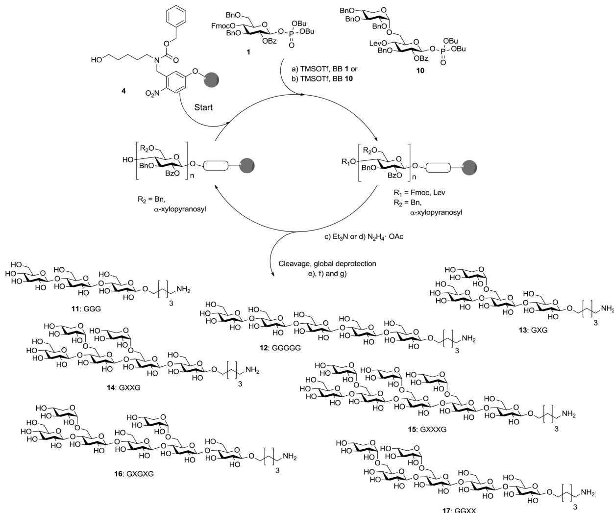
Scheme 3 Automated glycan assembly of XG oligosaccharides. Reagents and conditions: (a) 1 or 2 × 3.7 equiv. BB 1, TMSOTf, CH 2 Cl 2 , −30 °C (5 min) → −15 °C (30 min) (Module A); (b) 2 or 3 × 3.7 equiv. BB 10, TMSOTf, CH 2 Cl 2 , −35 °C (5 min) → −15 °C (35 min) (Module A); (c) 3 cycles of 20% NEt 3 in DMF, 25 °C (5 min) (Module B); (d) N 2 H 4 ·OAc (155 mM) in pyridine/AcOH/H 2 O 4 : 1 : 0.25, 25 °C (30 min) (Module C); (e) CH 2 Cl 2 , hν (305 nm); (f) NaOMe, THF/MeOH, 12 h; (g) H 2 , Pd/C, EtOAc/MeOH/H 2 O/HOAc, 12 h. 11: 28%; 12: 23%; 13: 15%; 14: 16%; 15: 2%; 16: 10%; 17: 9%. The letter code below the structures refers to a common nomenclature of XG oligosaccharides. 25
