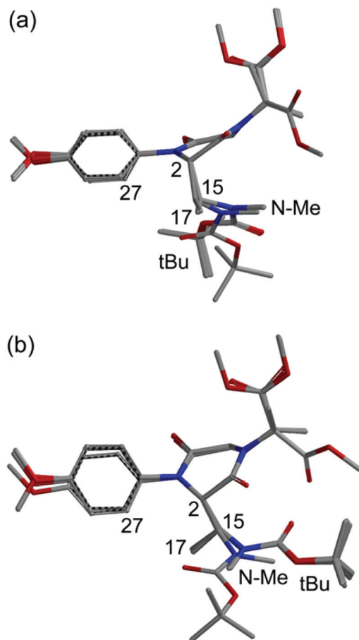
Fig. 2 Superposition of the first 9 low-energy structures of isomer C-2( S ) of compound 9 , calculated at the B3LYP/6-31G(d) level (a, more favored; b, less favored).
