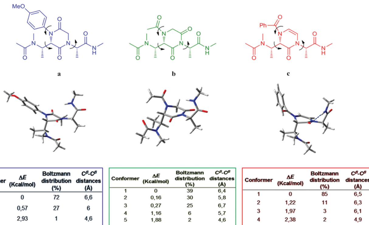
Fig. 4 Above: 2D structures of models a , b and c with their low energy conformers 3D images. Blue dotted line on model c represents the internal hydrogen-bond. Below: tables reporting the Boltzmann distributions and the C^\beta-C^\beta distances.
