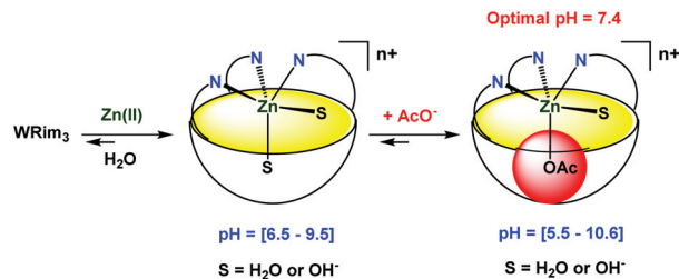
Scheme 3 Schematic representation of the coordination of Zn(II) and acetate by ligand \text{WRim}_3 in water. The variations of pH were obtained with nitric acid and sodium hydroxide.
