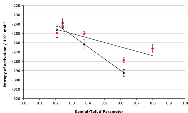
Fig. 7 The relationship between the entropy of activation and the Kamlet-Taft \beta parameter for the ionic liquids 5–9 (Table 1) at ca. \chi_{IL} 0.2 (♦) and 0.9 (♦), with the linear correlations having R^2 values of 0.671 and 0.955, respectively.
