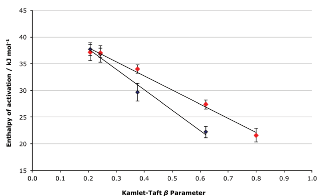
Fig. 6 The relationship between the enthalpy of activation and the Kamlet-Taft \beta parameter for the ionic liquids 5–9 (Table 1) at ca. \chi_{IL} 0.2 (♦) and 0.9 (♦), with the linear correlations having R^2 values of 0.992 and 0.983, respectively.
