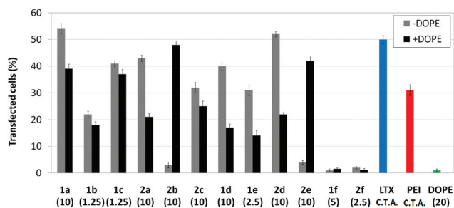
Fig. 11 In vitro transfection efficiency in COS-7 cells in the presence of nanocomplexes formulated with the pEGFP-C1 and \beta CD or \text{CA}_4 polycations 1a–f or 2a–f at their optimal concentration ( \mu\text{M} ) with and without DOPE (1 : 2 vector–DOPE molar ratio). Data for lipoplexes formulated with Lipofectamine® (LTX), and polyplexes formulated with polyethyleneimine (PEI) are also shown. C.T.A.: commercial transfection agent.
