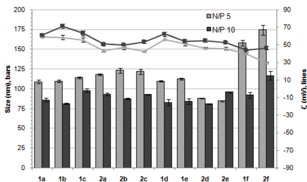
Fig. 5 Hydrodynamic diameter (bars, nm) and ζ potential (lines, mV) of complexes pDNA–polycationic amphiphilic derivatives determined by DLS and M3-PALS analysis.
