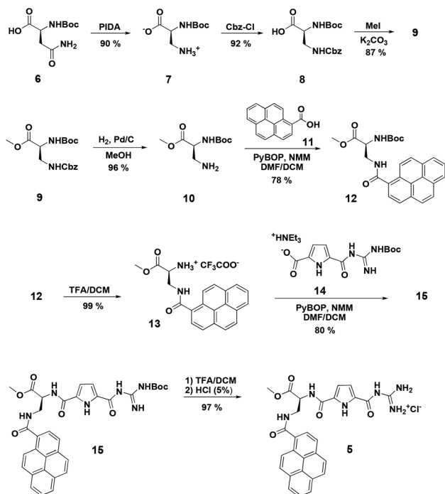
Scheme 2 Synthesis of the pyrene-functionalized amino acid 12 and the new DNA/RNA dye 5 (Boc = butyloxycarbonyl, PIDA = (diacetoxyiodo)-benzene, Cbz = carbobenzyloxy, MeOH = methanol, PyBOP = (benzotriazol-1-yloxy)tri pyrrolidinophosphonium hexafluorophosphate, TFA = trifluoroacetic acid, NMM = N -methylmorpholine, DCM = dichloromethane, NEt 3 = triethylamine).
