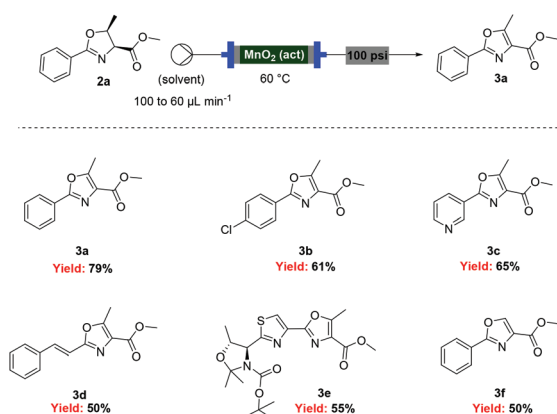
Scheme 4 Flow oxidation of aryl-oxazolines using activated MnO 2 .
