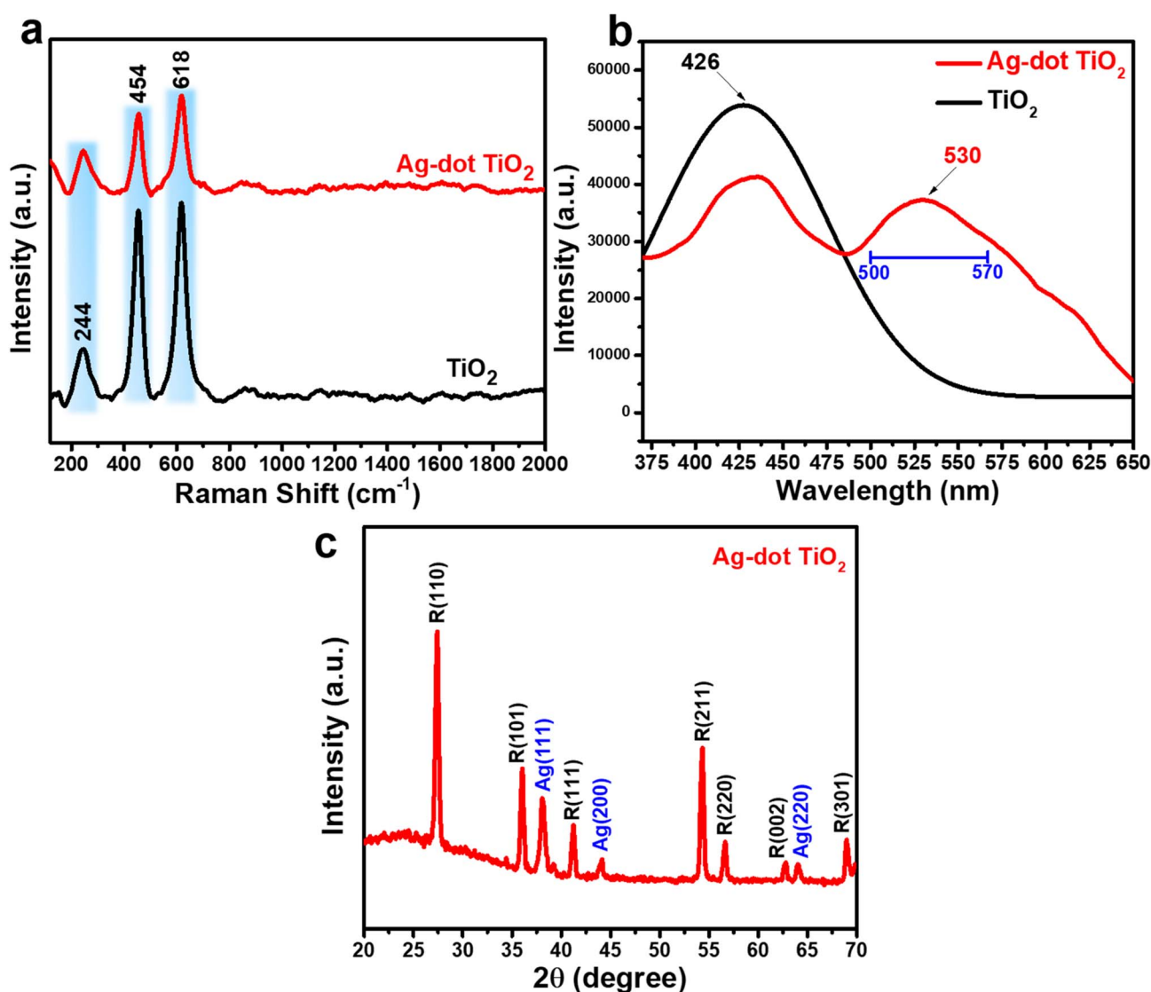
Fig. 2 Raman spectra (a) and PL spectra (b) of \text{TiO}_2 and Ag-dotted \text{TiO}_2 nanocomposite materials; XRD pattern of Ag-dotted \text{TiO}_2 nanocomposite materials (c).
