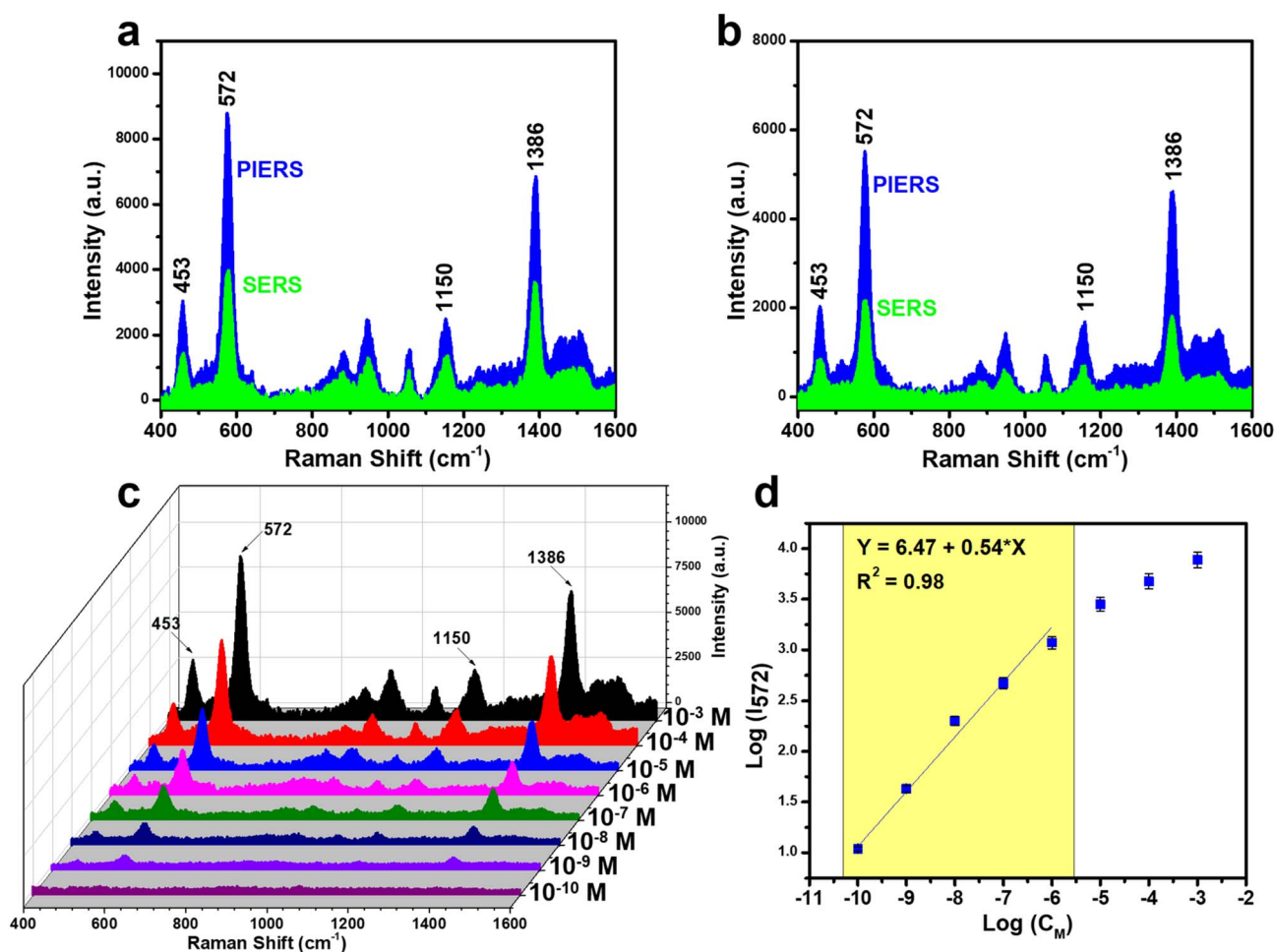
Fig. 9 Comparison of thiram sensing signals between PIERS and conventional SERS at concentrations of 10^{-3} M (a) and 10^{-4} M (b); PIERS spectra of thiram in the concentration range of 10^{-3} – 10^{-10} M (c); and the linear relationship between thiram concentration and signal intensity on a logarithmic scale (d).
