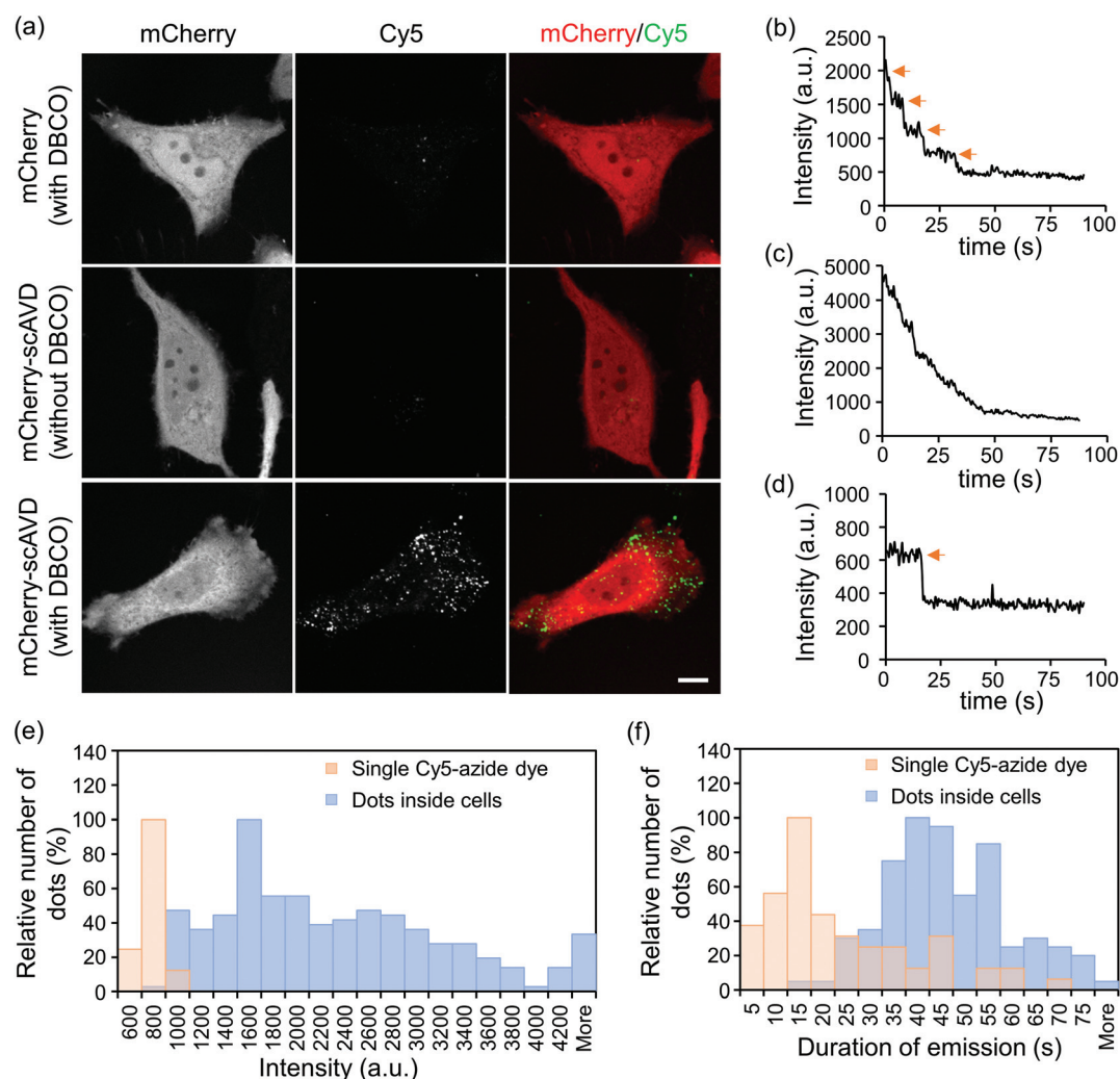
Fig. 3 Fluorescent nanoprobe probes showed increased brightness and enhanced photostability. (a) Confocal microscopy showed Cy5 dots formed in scAVD-overexpressing cells. Scale bar, 10 \mu\text{m} . (b–d) Time courses of fluorescence intensity changes of dots inside cells (b and c) and a single Cy5-azide dye on a glass bottom dish located outside cells (d) during photobleaching. Orange arrows indicate the photobleaching steps. (e) Histogram showing the distribution of fluorescence intensity of Cy5 dots ( n = 248 ) and single Cy5-azide dye ( n = 156 ). (f) Histogram showing the distribution of the duration of emission of Cy5 dots ( n = 118 ) and single Cy5-azide dye ( n = 63 ) before they were photobleached.
