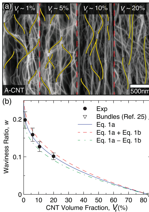
Fig. 3 Evolution of the CNT waviness with packing. (a) Cross-sectional scanning electron microscopy (SEM) micrographs of CNT arrays at volume fractions ( V_f ) ranging from \sim 1 – 20 vol.% CNTs showing the reduction in CNT waviness. (b) Plot demonstrating that the waviness ratio ( w ) can be reduced by \sim 50\% by increasing V_f from \sim 1 vol.% CNTs to \sim 20 vol.% CNTs.
