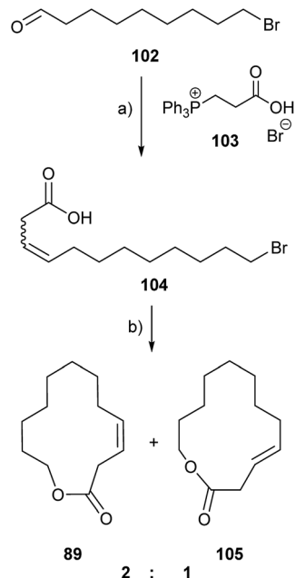
Fig. 14 Synthesis of ( Z )-dodec-3-en-12-olide ( 89 ). (a) NaHMDS; (b) K_2CO_3 , KI.
