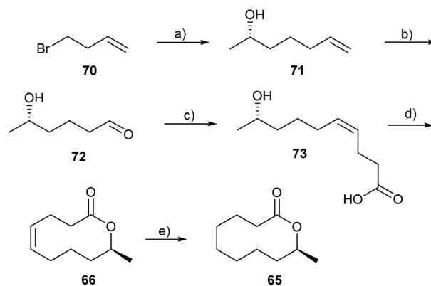
Fig. 9 Synthesis of ( S )-phoracantholide I ( 65 ) and ( S )-phoracantholide J ( 66 ). 101 (a) Mg, CuCN, ( S )-propylene oxide; (b) K_2O_8O_4 , NaIO 4 ; (c) NaHMDS, [Ph 3 P(CH 2 ) 3 COOH]Br (Z : E = 95 : 5); (d) dipyridyl disulfide, AgClO 4 ; (e) H 2 , Pd/C.
