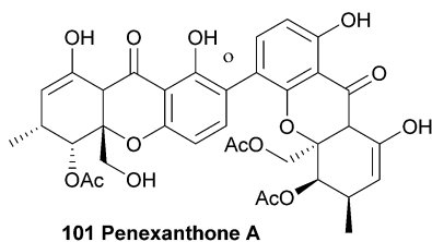
101 Penexanthone A
