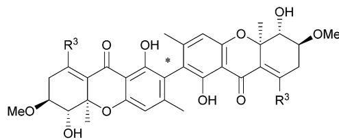
78 Ascherxanthone A; R_1 = \text{OMe}, R_2 = \text{Me}, R_3 = H (relative stereochem.) 79 Ascherxanthone B; R_1 = \text{OMe}, R_2 = \text{Me}, R_3 = \text{OH} (relative stereochem.) 80 TMC 315A; R_1 = \text{Me}, R_2 = \text{OMe}, R_3 = \text{OH} (no stereochemistry known) 81 TMC 315A 2 ; R_1 = \text{OMe}, R_2 = \text{Me}, R_3 = \text{OH} (no stereochemistry known)
