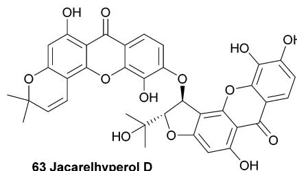
63 Jacarelhypers D
