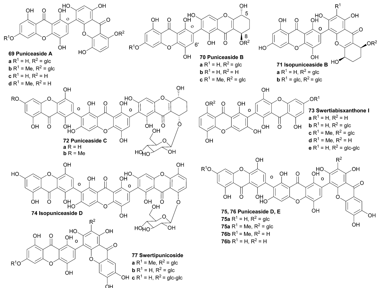
Fig. 2 Puniceaside and swertiabixanone derivatives (absolute stereochemistries shown).
