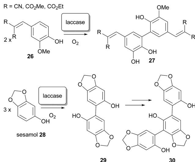
Scheme 4 The synthetic usage of laccase enzymes in biaryl-linked dimers.
