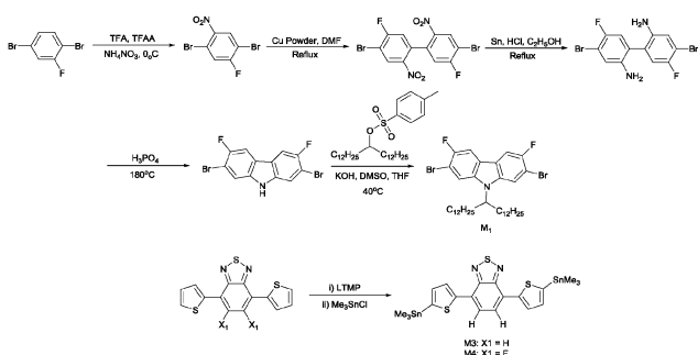
Scheme 1 Synthetic routes to the final monomer products: M1 , M3 and M4 . M2 was synthesised using previously established literature procedures.
