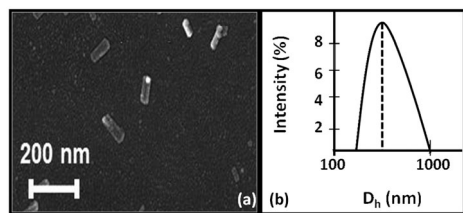
Fig. 1 (a) SEM image and (b) DLS size distribution plot of heptamolybdate SOMs.
