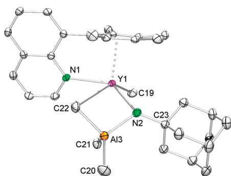
Fig. 5 Molecular structure of 7 . Atoms are represented by atomic displacement ellipsoids set at the 50% level. Selected bond distances [Å] and angles [deg]: \text{Y1}-\text{C19} 2.392(2) , \text{Y1}\cdots\text{C22} 3.006(2) , \text{Y1}-\text{N1} 2.527(2) , \text{Y1}-\text{N2} 2.428(2) , \text{Y1}\cdots\text{Ct1} 2.366 , \text{Y1}\cdots\text{Al3} 3.0417(6) , \text{Al3}-\text{C20} 1.964(2) , \text{Al3}-\text{C21} 2.007(2) , \text{Al3}-\text{C22} 2.022(2) , \text{Al3}-\text{N2} 1.920(2) , \text{Y1}-\text{N2}-\text{C23} 126.9(1) , \text{Y1}-\text{N2}-\text{Al3} 87.98(7) , \text{C19}-\text{Y1}-\text{C22} 144.61(7) , \text{N1}-\text{Y1}-\text{N2} 140.16(6) , \text{C19}-\text{Y1}-\text{N2} 103.26(7) , \text{C19}-\text{Y1}-\text{N1} 95.24(7) , \text{C22}-\text{Y1}-\text{N1} 78.49(6) , \text{Y1}-\text{N2}-\text{Al3}-\text{C22} -55.70(9) .
