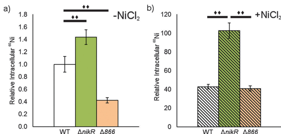
Fig. 8 The impact of HPG27_866 on total nickel. The levels of total cellular nickel was measures in wild-type, Δ nikR and Δ 866 H. pylori G27 using ICP-MS. Each strain was grown overnight without (a) or with (b) a media supplement of 10 μM NiCl 2 . Counts from 24 Mg were used as an internal control for differences in cell number for each sample. The data represent the average values from five biological replicates and significant changes ( P < 0.01 ) between conditions are marked with a double diamond.
