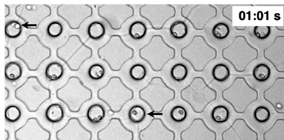
Fig. 4 Cell loading in a VIA devices showing both single and two cell occupancy after at a time of 1 min after commencement of loading at 0.1 \mu\text{l min}^{-1} . For \sim 60 s loading time, although the overall microwell occupancy increases, the relative proportion of single to two cell occupancy decreases.
