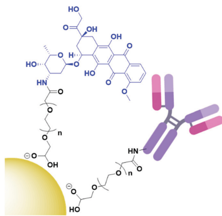
Fig. 3 Structure of antibody directed doxorubicin (blue) AuNPs, with both the payload and antibody conjugated through a PEG (black) linker (adapted from ref. 54).
