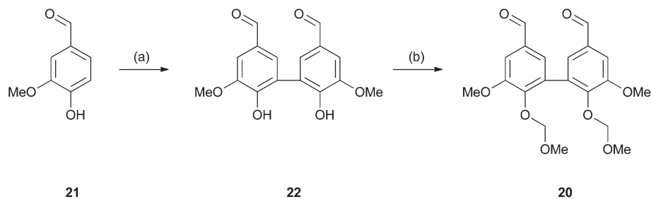
Scheme 5 The synthesis monomer 20 . Reagents and conditions: (a) \text{K}_2\text{S}_2\text{O}_8 , (\text{NH}_4)_2\text{Fe}(\text{SO}_4)_2 \cdot \text{H}_2\text{O} , \text{H}_2\text{O} , 90^\circ\text{C} , 15 min, 82%. (b) Dimethoxymethane, \text{AcCl} , \text{ZnBr}_2 (cat.), toluene, r.t. 3 hours then 22 , Hunig's base, DMF, 24 hours, r.t., 64%.
