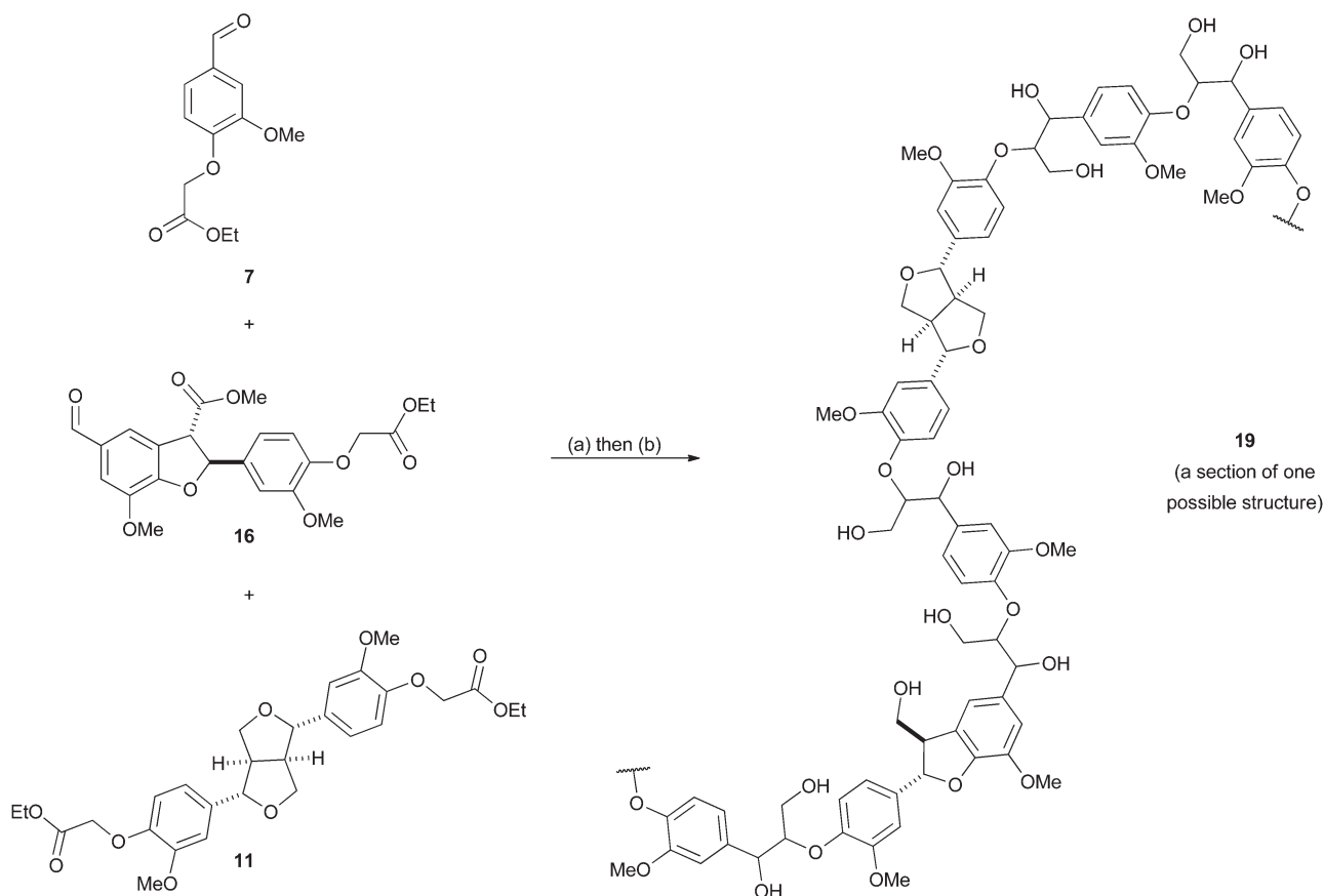
Scheme 4 The synthesis of a softwood lignin model polymer 19 . Reagents and conditions: (a) LDA, THF, -78 °C to 0 °C, 1 h. (b) \text{NaBH}_4/\text{MeOH} , EtOH, 50 °C, 1 h, 40% over 2 steps.
