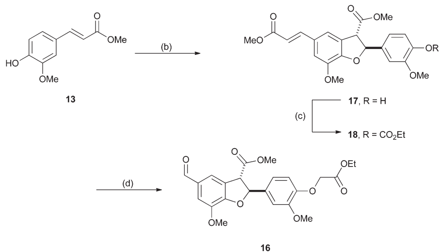
Scheme 3 The synthesis of the \beta -5 monomer 16 . Reagents and conditions: (b) HRP, \text{H}_2\text{O}_2 , \text{H}_2\text{O}/\text{MeOH} (87 : 13), pH 3, 37 °C, 10 min, 43%. (c) Ethyl iodoacetate, \text{K}_2\text{CO}_3 , acetone, reflux, 16 h, 72%. (d) \text{RuCl}_3 \cdot x\text{H}_2\text{O} (~0.2 mol%), \text{NaIO}_4 , \text{EtOAc}/\text{MeCN}/\text{H}_2\text{O} , 0 °C to r.t., 3 h, 70%.
