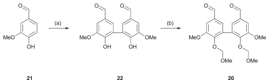
Scheme 5 The synthesis monomer 20 . Reagents and conditions: (a) K_2S_2O_8 , (NH_4)_2 \cdot Fe(SO_4)_2 \cdot H_2O , H_2O , 90^\circ C , 15 min, 82%. (b) Dimethoxymethane, AcCl , ZnBr_2 (cat.), toluene, r.t. 3 hours then Hunig's base, DMF , 24 hours, r.t., 64%.
