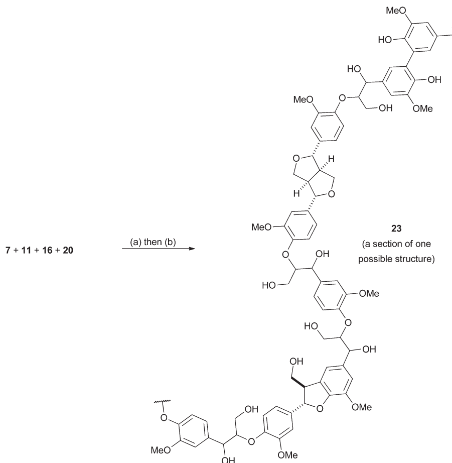
Scheme 6 The synthesis of a phenolic softwood lignin model polymer 23 . Reagents and conditions: (a) LDA , THF , -78^\circ C to 0^\circ C , 1 h. (b) NaBH_4 /MeOH, EtOH, 50^\circ C , 1 h, 32% over 2 steps.
