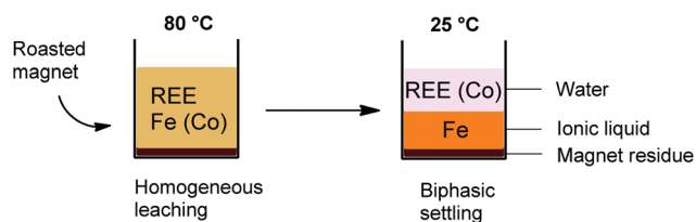
Fig. 8 Schematic overview of the biphasic leaching-settling process using a thermomorphonic ionic liquid. The [Hbet][Tf 2 N]–H 2 O mixture forms one homogeneous phase at 80 °C and forms two phases at room temperature.
