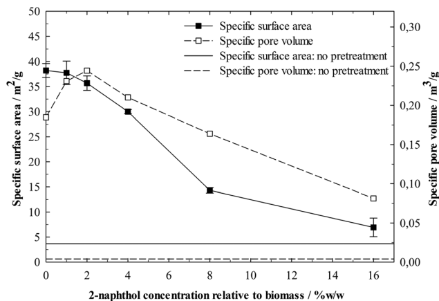
Fig. 9 BET specific surface area and BJH specific pore volume of isolated lignin residues from spruce after a pretreatment with different concentrations of 2-naphthol. Horizontal lines represent specific surface area and pore volume of lignin isolated from non-pretreated spruce.
