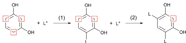
Fig. 3 Reaction scheme adapted from Lora and Wayman 1 showing the first (1) and second (2) reaction of resorcinol with a lignin carbocation (L+). Positions most reactive towards electrophilic aromatic substitution are highlighted.
