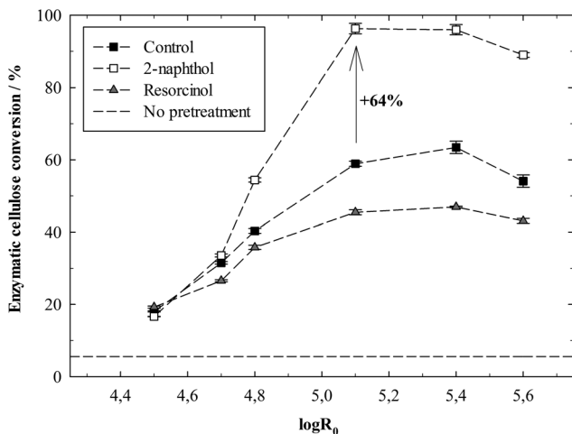
Fig. 4 Cellulose conversion/glucose yields in the enzymatic hydrolysis of spruce after autohydrolysis pretreatments at different severities with 2-naphthol (4.7%w/w of biomass), resorcinol (1.8%w/w of biomass) and no additive (control). Yields do not account for cellulose degradation during pretreatment. Hydrolysis conditions: 1%w/w cellulose, 60 FPU g^{-1} cellulose.
