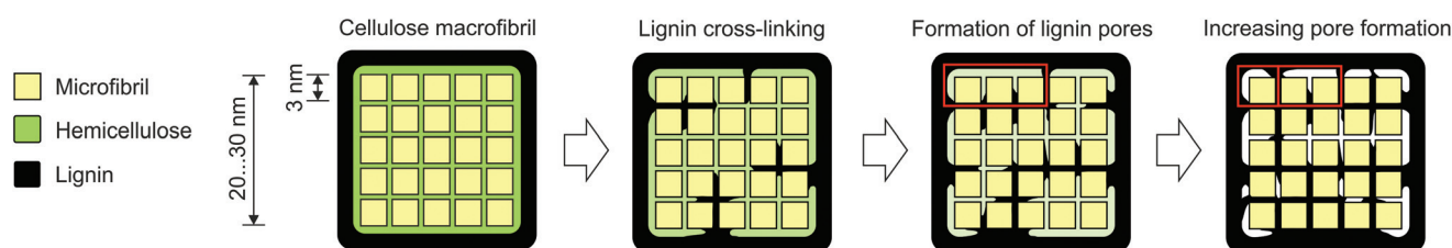
Fig. 11 Scheme denoting a possible way for the formation of porous lignin structures by cross-linking within a cellulose macrofibril during pretreatment. Advancing cross-linking increases the amount of pores while decreasing their average diameter (highlighted by red squares).
