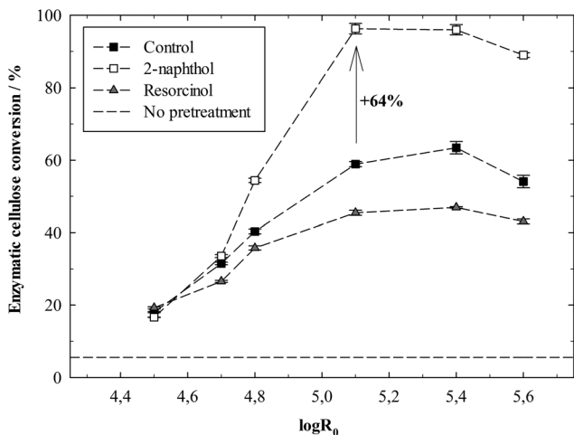
Fig. 4 Cellulose conversion/glucose yields in the enzymatic hydrolysis of spruce after autohydrolysis pretreatments at different severities with 2-naphthol (4.7%w/w of biomass), resorcinol (1.8%w/w of biomass) and no additive (control). Yields do not account for cellulose degradation during pretreatment. Hydrolysis conditions: 1%w/w cellulose, 60 FPU g -1 cellulose.
