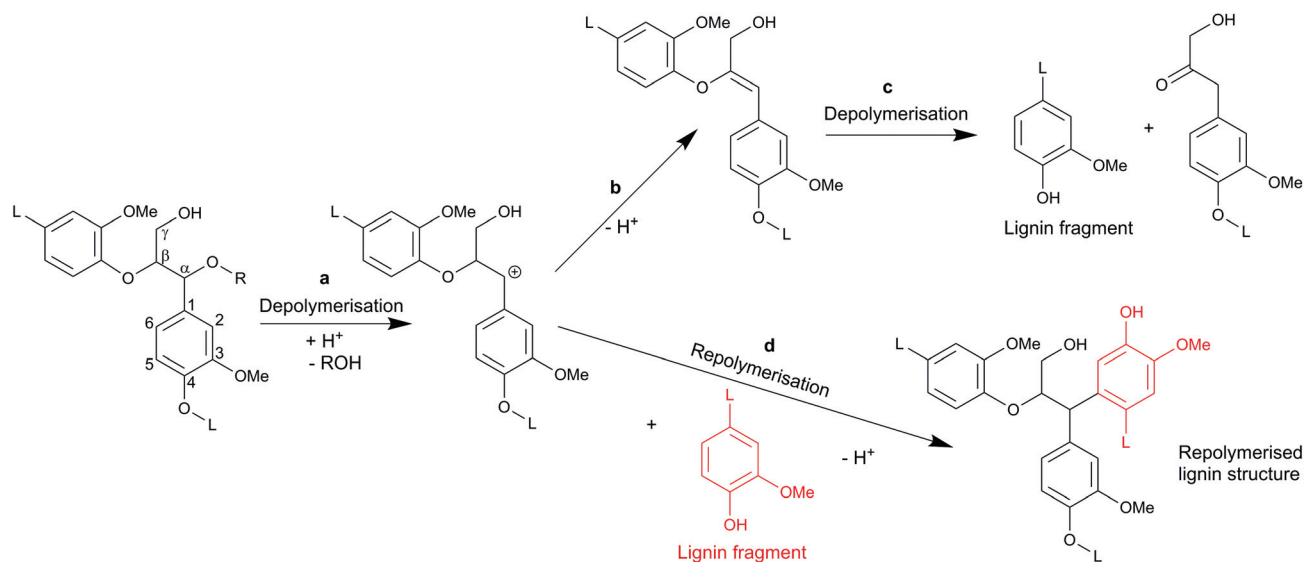
Fig. 1 Scheme for reactions of lignin in acidic media adapted from Voitl et al. 15 (a) cleavage of β-O-4 bond and formation of carbocation; 16 (b) elimination of β-proton giving rise to an enol ether; 16 (c) acid hydrolysis of enol ether; 16 (d) repolymerisation reaction. 17
