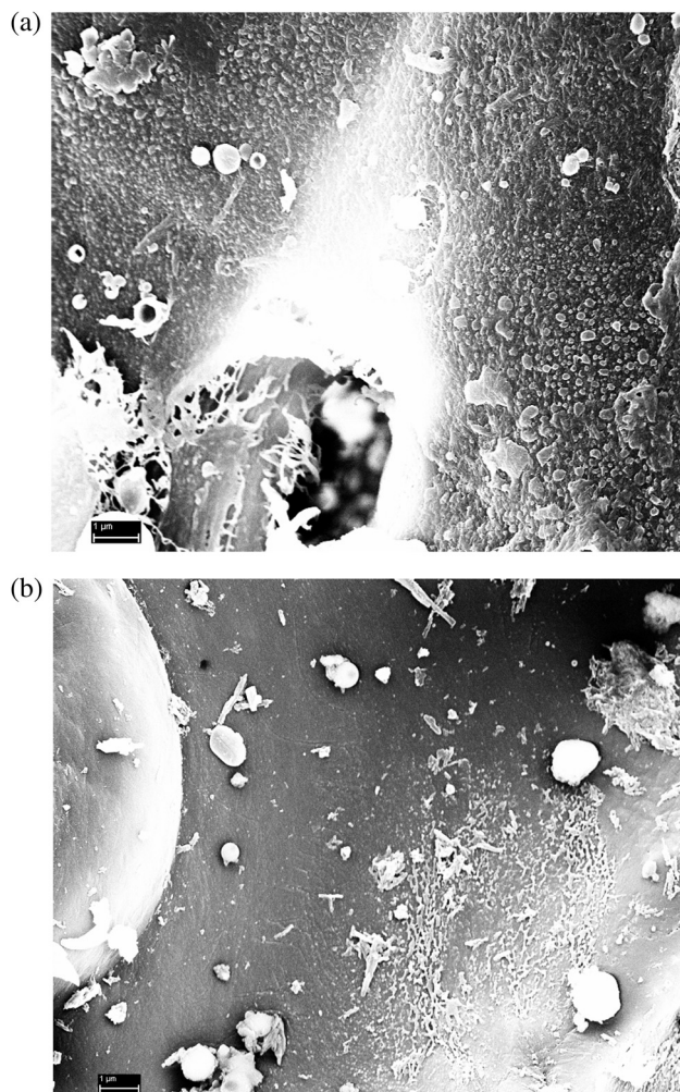
Fig. 12 SEM images of lignin residues isolated from spruce pretreated without (top) and with 16%w/w 2-naphthol relative to biomass (bottom).
