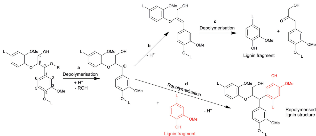
Fig. 1 Scheme for reactions of lignin in acidic media adapted from Voittl et al. 15 (a) cleavage of \beta -O-4 bond and formation of carbocation; 16 (b) elimination of \beta -proton giving rise to an enol ether; 16 (c) acid hydrolysis of enol ether; 16 (d) repolymerisation reaction. 17
