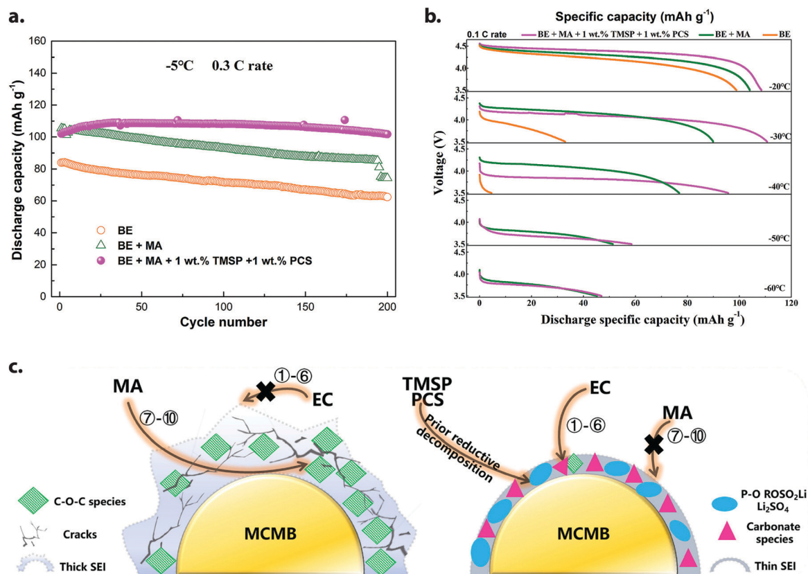
Fig. 8 (a) Cycling performance of MCMB||LiNi 0.5 Mn 1.5 O 4 full cells (3.5–4.9 V) at -5^{\circ}\text{C} and 0.3C rate in commercially-available baseline electrolyte (BE), a modified electrolyte containing methyl acetate (BE + MA) and the preceding electrolyte with tris(trimethylsilyl)phosphite and 1,3-propanediol cyclic sulfate additives (BE + MA + 1 wt.% TMSP + 1 wt.% PCS). (b) Discharge characteristics of the above cell designs at -20 to -60^{\circ}\text{C} , following a 0.5C charge at room temperature. (c) Proposed working mechanism of the aforementioned phosphite and sulfate additives in this system, based on XPS analysis of cycled MCMB anodes. Formation of a thin, robust SEI prevents continuous decomposition of methyl acetate and resists Li dendrite growth during low-temperature charge. Reprinted/adapted from ref. 74 with permission from Elsevier.
