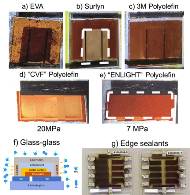
Fig. 17 Example of encapsulation (a)–(e) various polymers. Reproduced with permission. 181 Copyright 2018, The Royal Society of Chemistry. (f) Glass–glass, 186 Copyright 2022, American Chemical Society. Licensed under CC BY-NC-ND 4.0. (g) Edge sealants. Reproduced with permission. 184 Copyright 2024 International Solar Energy Society.
