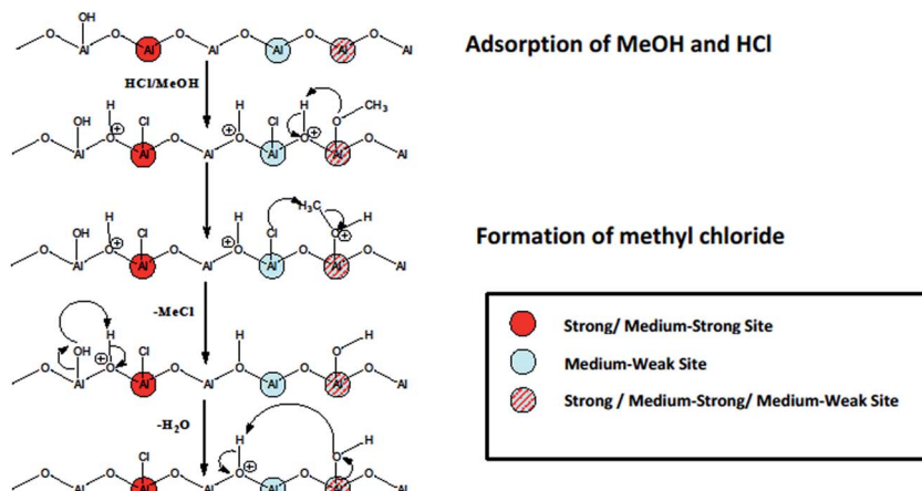
Fig. 1 A schematic representation of the site-selective formation of methyl chloride over \eta -alumina. The red circles represent a strong/medium-strong Lewis acid site; the blue circles represent a medium-weak Lewis acid site; the red/blue shaded circles represent a strong/medium-strong/medium-weak Lewis acid site. The definition and form of these sites is described in ref. 9.
