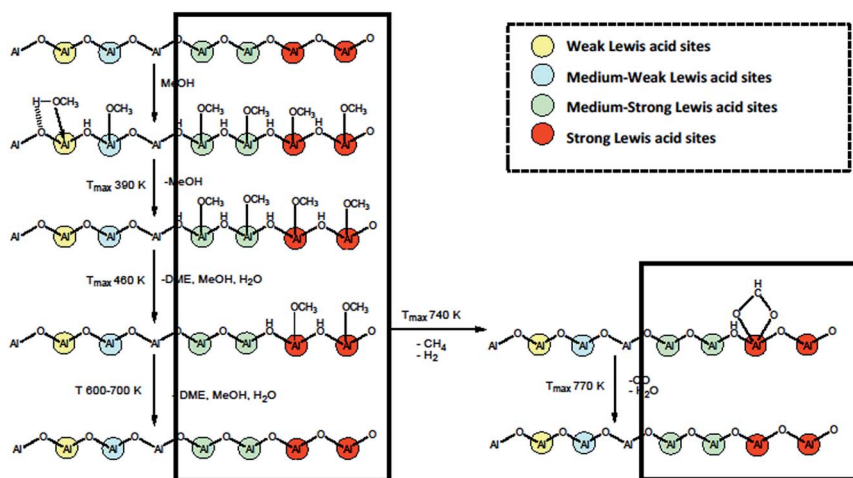
Fig. 10 Proposed methanol transformations during temperature programming of an \eta -alumina catalyst doped with 1.0 \text{ mmol } g_{\text{(cat)}}^{-1} of a Group 1 metal salt. The areas bounded by the solid black line represent chemistry no longer accessible due to the Group 1 metal “capping” the strong and medium-strong Lewis acid sites. This mechanism is a variation on that proposed for the reaction of methanol on \eta -alumina, 11 that is reproduced with permission from Lundie et al. , J. Phys. Chem. B , 2005, 109 , 11592. Copyright 2005 American Chemical Society.
