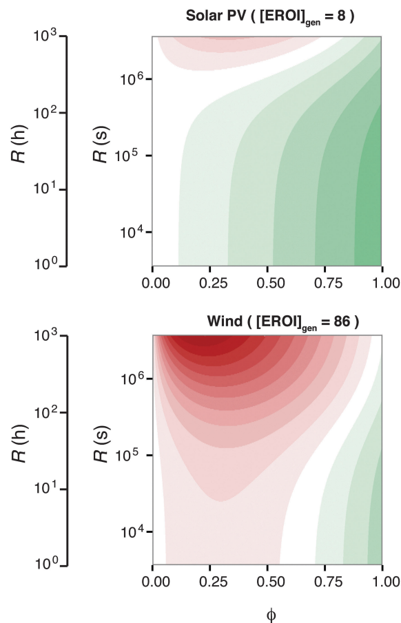
Change in [\text{EROI}]_{\text{grid}} when building RHFC storage instead of curtailing
