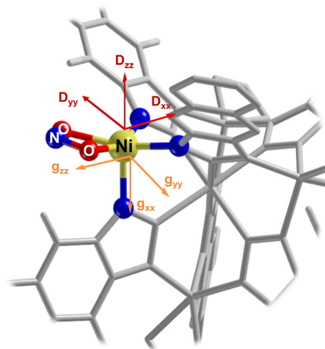
Fig. 3 Geometry optimized periodic structures at B3LYP-D3/pob-TZVP-rev2 of Ni-MFU-4l- \text{NO}_2 . The computed g - and D -tensor frames are also reported.
