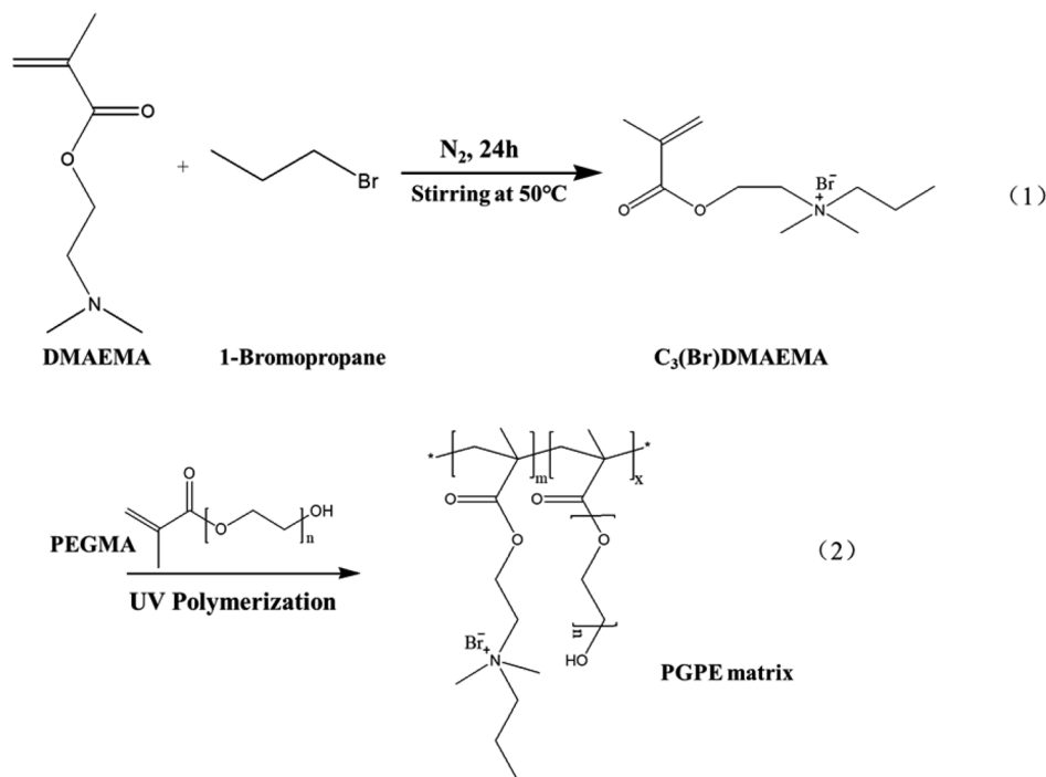
Scheme 1 Synthesis of the PGPE matrix.
