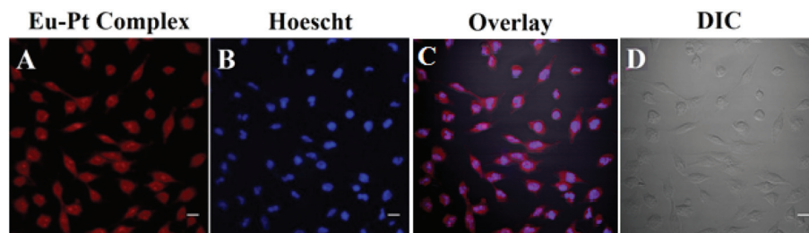
Fig. 3 Confocal laser scanning fluorescence microscopic images of the HeLa cells treated with the Eu–Pt 2 complex (25 \mu\text{M} ) after 4 h of incubation and Hoechst 33258 dye (5 \mu\text{g mL}^{-1} ): (A) cells incubated with the Eu–Pt 2 complex; (B) incubated with the Hoechst 33258 dye for staining nuclei, which show blue emission; (C) merged images showing nuclear and cytosolic localization of the complex; (D) DIC images. Scale bar = 20 \mu\text{m} .
