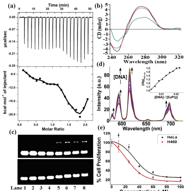
Fig. 2 (a) ITC plot profile for the interaction of Eu–Pt 2 (0.1 mM) with CT-DNA (0.01 mM) in 5 mM Tris-HCl/NaCl buffer (pH 8.5) at 30 °C. The top panel represents the raw data for 20 injections of 2 \mu L each. The bottom panel shows the amounts of heat evolved on interaction of the Eu–Pt 2 complex with CT-DNA against the molar ratio of Eu–Pt 2 complex to CT-DNA. Data were fitted by a sequential binding site model. (b) CD spectra of CT-DNA in the presence of EuL and Eu–Pt 2 in Tris-HCl buffer medium. (c) Agarose gel electrophoresis of SC pUC19 DNA after incubation with EuL and Eu–Pt 2 in 50 mM Tris-HCl buffer at 37 °C for 16 h. Lane 1: DNA control, lanes 2–8 (10, 15, 20, 40, 60, 80 and 100 \mu M complexes respectively). (d) Luminescence spectra of Eu–Pt 2 ( \lambda_{\text{ex}} = 330 nm) with the addition of CT-DNA in 5 mM Tris-HCl buffer. Inset: the relative emission intensity ( I/I_0 ) of 1 at 615 nm vs. [DNA]/[Eu–Pt 2 ] ratio. (e) Cell viability plots showing the cytotoxicity of the Eu–Pt 2 complex with HeLa and H460 cells on 16 h incubation by MTT assay.
