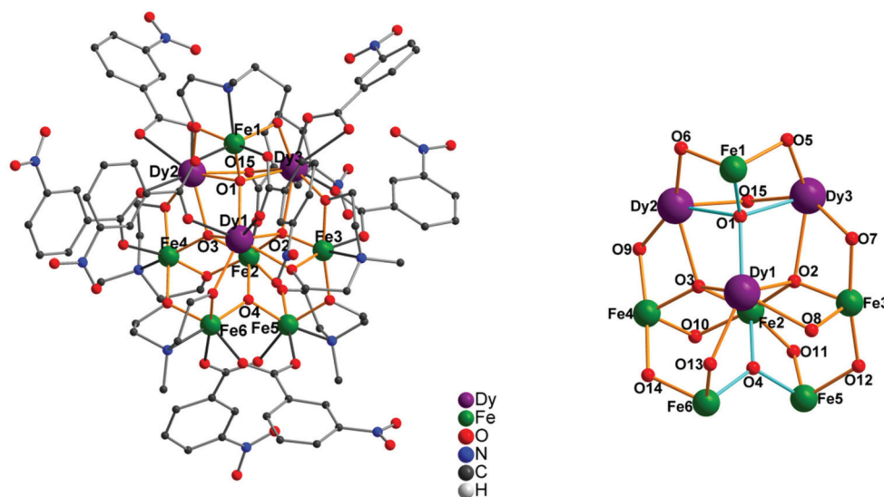
Fig. 2 Molecular structure (left) and core (right) of the coordination cluster in [\text{Fe}_6\text{Dy}_3(\mu_4\text{-O})_3(\mu_3\text{-O})(\text{mdea})_5(m\text{-NO}_2\text{C}_6\text{H}_4\text{COO})_9]\cdot 3\text{MeCN} ( 4 ). Organic H atoms have been omitted for clarity.
