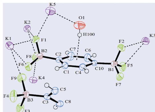
Fig. 1 ORTEP-plot of the asymmetric unit of the title compound 2 with ellipsoids plotted at the 50% probability level. Short K...F, K...O contacts and OH... \pi interactions are drawn as dashed lines. Colour codes in the electronic version of the paper: carbon (blue), boron (light brown), fluorine (green), potassium (violet) and oxygen (red). Hydrogen atoms are also drawn as small spheres.
