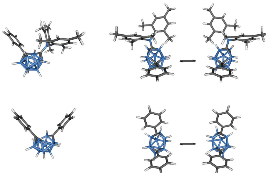
Fig. 15 Optimised geometries of [2]^{2-} (top) and [5]^{2-} (bottom) and the fluctual processes.
