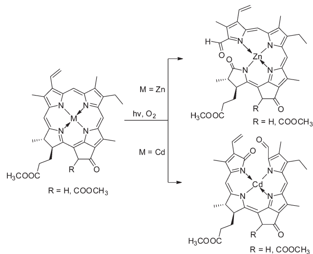
Fig. 6 Photo-oxygenolysis of Zn(II)- and Cd(II)-(pyro)phorboidates allows the efficient preparation of 1-formyl-19-oxobilins with regio-selective cleavage of the macrocycle at the 'western' \delta - meso position or at the 'northern' \alpha - meso position, respectively.
