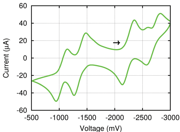
Fig. 5 Cyclic voltammogram for (4,4'-bipy){Ti(N[ t Bu]Ar) 3 ] 2 in THF with a sweep rate of 800 mV s -1 referenced vs. Fc/Fc + with [N n Bu 4 ][B(C 6 F 5 ) 4 ] (0.2 M) as the supporting electrolyte. The arrow signifies the rest potential and the direction of the sweep.
