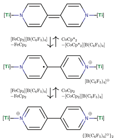
Fig. 6 Isolable in three states of charge, the figure depicts schematically (4,4'-bipy){Ti(N[ t Bu]Ar) 3 ] 2 , its mono-cation, and di-cation, the latter cations both having been isolated as perfluoro-tetraphenyl borate salts.
