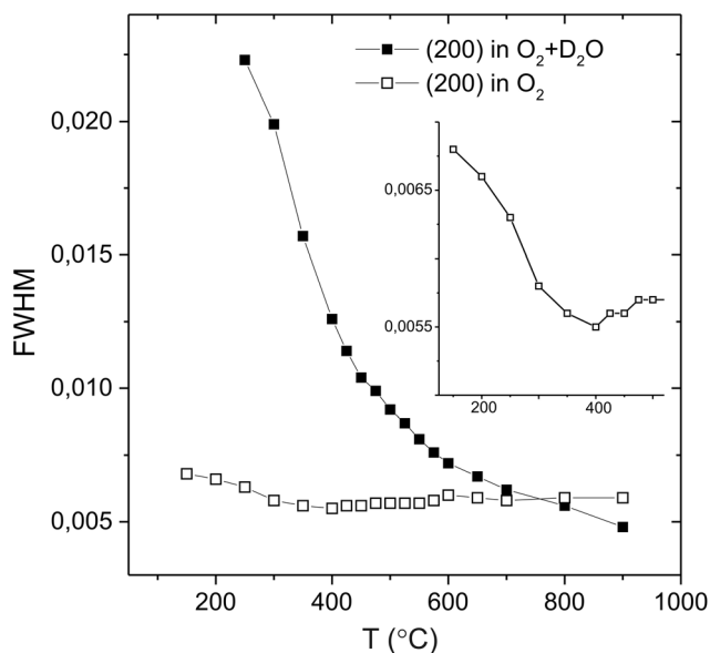
Fig. 2 Analysis of the FWHM of the intensity in the region of the cubic (200) reflection in O_2 and O_2 + D_2O(g) atmospheres. Inset shows a close-up of the dry O_2 behaviour revealing broadening linked to the appearance of the Imma phase at T < 300 °C.
