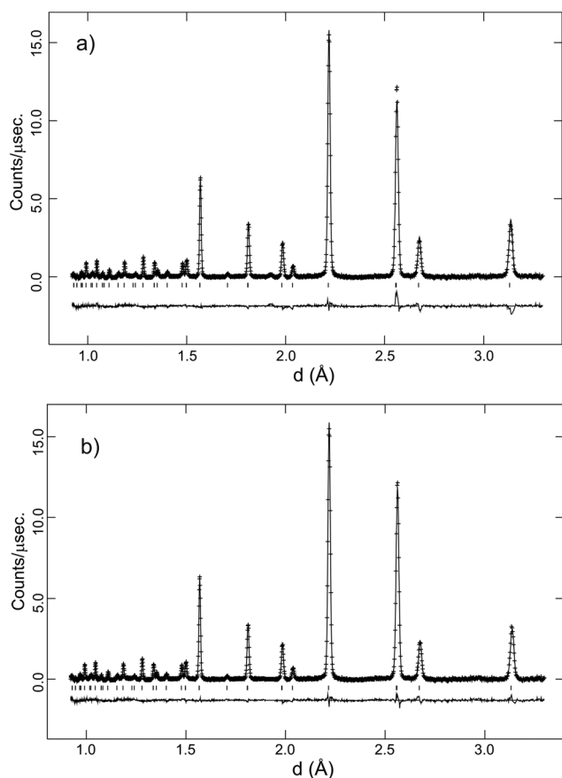
Fig. 8 (a) Rietveld fit achieved, with no deuterium position defined, to the 700 °C, \text{O}_2 + \text{D}_2\text{O}_{(\text{g})} data for \text{BaCe}_{0.8}\text{Y}_{0.2}\text{O}_{3-\delta} . (b) Rietveld fit achieved with the deuterium position defined at the 36f site to the same data. Crosses are observed data, lines are the calculated profile and difference plot. Tick marks indicate reflection positions for the R\bar{3}c structural model.
