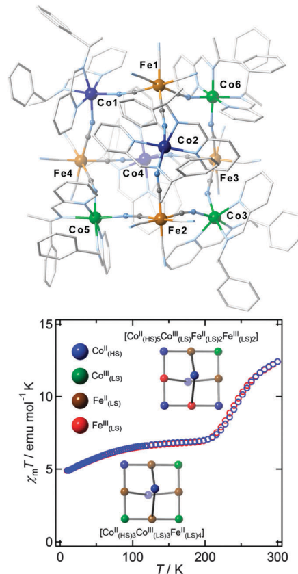
Fig. 9 (top) Representation of the molecular structure of [\text{NET}_4]_2\{[\text{Co}(\text{L}^{\text{R}})]_6[\text{Fe}(\text{CN})_6]_4\}[\text{BF}_4] \cdot 17\text{CH}_3\text{OH} \cdot 12\text{H}_2\text{O} ( 29 ) at T = 100 \text{ K} . Hydrogen atoms, tetrafluoroborate and lattice-solvent molecules are omitted for clarity. Fe(II), Co(III), Co(II), N and C atoms are indicated in brown, green, dark blue, light blue and light grey, respectively. (bottom) \chi T versus T data cooling (blue dots) and heating (red dots) the sample, together with the diagrams of the spin state of each metal ion. Reprinted with permission from ref. 79. Copyright (2014) American Chemical Society.
