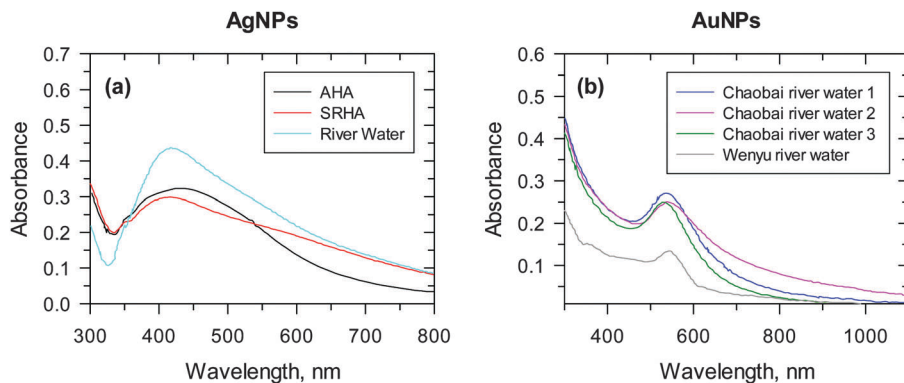
Fig. 6 UV-vis spectra of nanoparticles formed under river water conditions. (a) Ag nanoparticles, 4 \text{ mg L}^{-1} Suwannee river humic acid (SRHA) (red line), or 4 \text{ mg L}^{-1} C/L Aldrich humic acid (AHA) (black line) upon exposure to stimulated sunlight in the CPS+ reactor for 20 min. ( [\text{Ag}^+] = 1 \times 10^{-4} \text{ M} ; pH 8.0). (Adapted with permission from ref. 28, copyright American Chemical Society). (b) Au nanoparticles under natural sunlight. (Cumulative parabolic aluminized reflector (PAR) light = 12.48 \text{ E m}^{-2} ). (Adapted with permission from ref. 30, copyright American Chemical Society).
