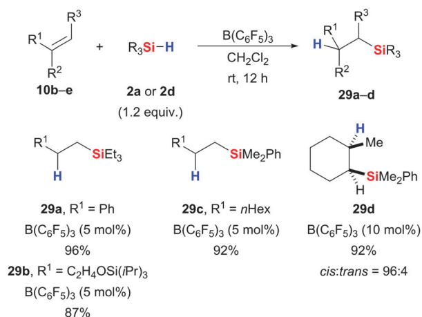
Scheme 14 B(C 6 F 5 ) 3 -catalysed hydrosilylation of alkenes by Gevorgyan.
