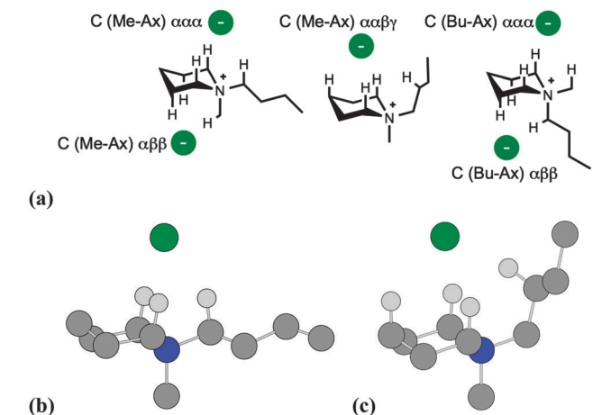
Fig. 3 (a) Primary cation-anion interactions for chair conformers of [C_4C_1\text{pip}]\text{Cl} , 2 . Structures of the: (b) 'C (Me-Ax) \alpha\alpha\alpha 1', and; (c) 'C (Me-Ax) \alpha\alpha\beta\gamma ' ion pair conformers of 2 , showing primary H-bond interactions. All other hydrogen atoms are omitted, for clarity.
