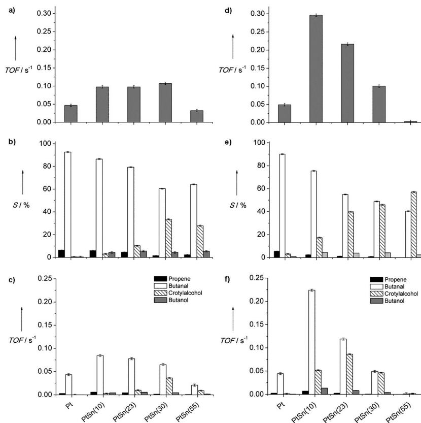
Fig. 2 TOF (s -1 ) with respect to the conversion of crotonaldehyde, selectivity and TOF (s -1 ) with respect to the formation of the individual products formed by the hydrogenation of crotonaldehyde as a function of Sn content for the as-prepared (a–c) and the pre-reduced catalysts (d–f), respectively. The gas flow rate was set to 50 ml min -1 containing 1 vol% crotonaldehyde, 20 vol% H 2 and N 2 as balance. All measurements were conducted under isothermal conditions at 80 °C.
