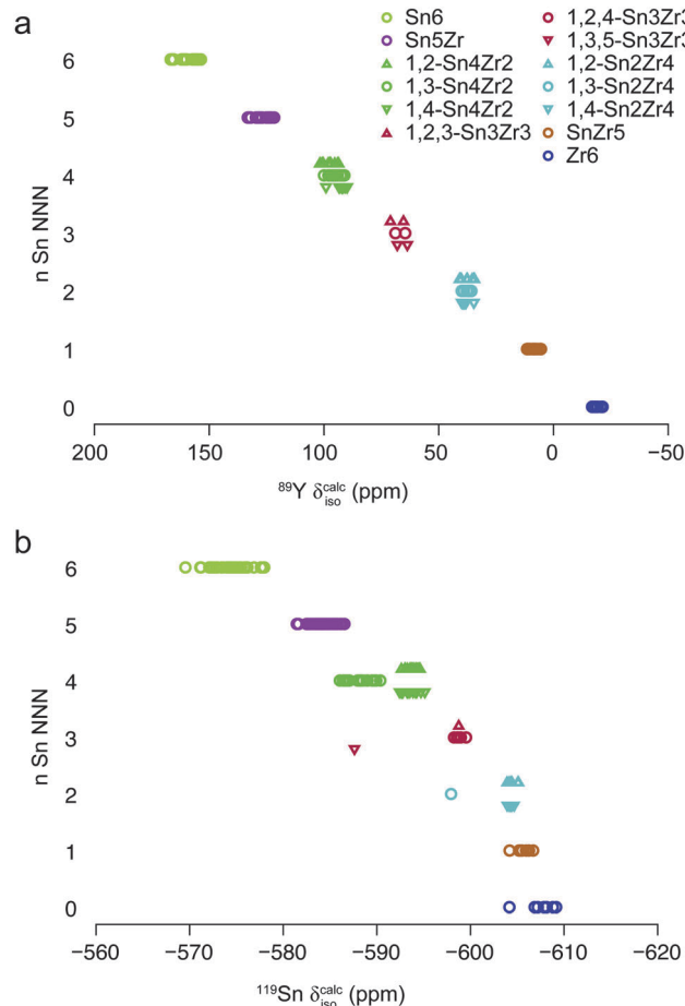
Fig. 3 Plots showing the (a) ^{89}Y and (b) ^{119}Sn calculated isotropic chemical shifts, \delta_{iso}^{calc} , as a function of the number, n , of Sn NNN for Y_2(Zr,Sn)_2O_7 model pyrochlores with local environments as described in the ESI.†
