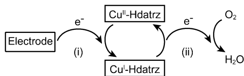
Scheme 2 Simplified electron transfer steps in the Cu-Hdatrz/KB system: (i) electron transfer from the electrode/KB to Cu II -Hdatrz and (ii) electron transfer from Cu I -Hdatrz to O 2 (the ORR step).
