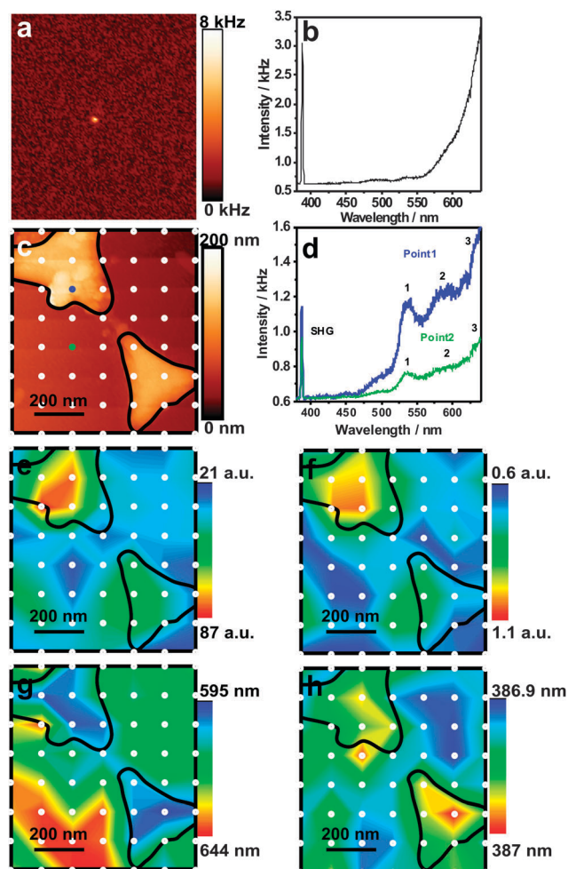
Fig. 4 Hyperspectral SNOM mapping of the nanotriangles. (a) The nonlinear optical image when a sharp Au tip scans through the laser focus. (b) A spectrum collected from an excited Au tip, (c) topography of nanotriangles, (d) two nonlinear spectra obtained from the Au–tip–nanotriangle junction at two different positions (marked in blue and green colours) that are indicated in image (c) by the blue and green circles, (e) SNOM 2PPL intensity map, (f) SNOM SHG intensity map, (g) peak 2 position variation map, (h) SHG peak variation map. The white dotted matrix ( 7 \times 8 ) marks the positions where tip-enhanced nonlinear spectra were taken. Spectral integration time: 60 s.
