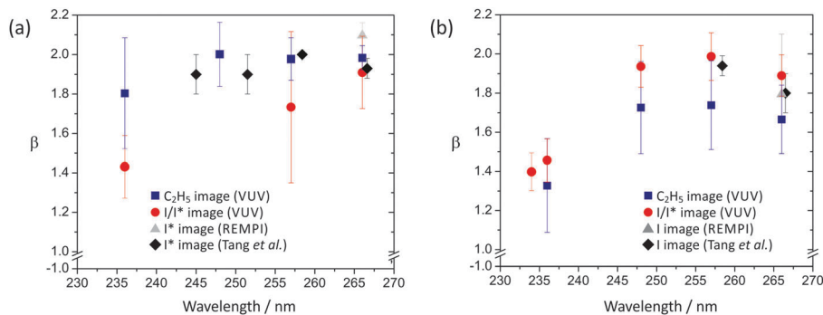
Fig. 10 Anisotropy parameters for (a) C_2H_5 + I^* , and (b) C_2H_5 + I dissociation channels following ethyl iodide photolysis at wavelengths in the UV. Note the expanded vertical scale.
