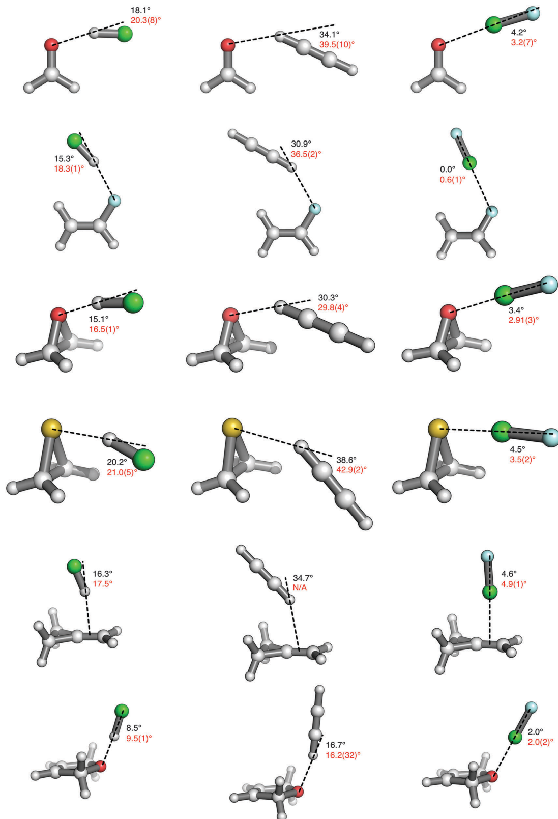
Fig. 2 Geometries of the B \cdots HCl (left column), B \cdots HCCH (centre column) and B \cdots ClF (right column) complexes. Black text denotes the theoretical CCSD(T)-F12b deviations from collinearity ( \theta ), red text (lower) are experimental. 12,19,24,26,29,32–36,38,39
