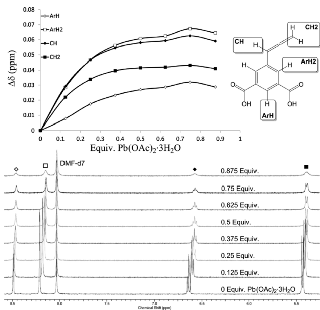
Fig. 2 Titration isotherm and ^1\text{H-NMR} spectroscopic titration stack plot for the interaction between \text{H}_2\text{abd} and \text{Pb}(\text{OAc})_2 \cdot 3\text{H}_2\text{O} in \text{DMF-d}_7 .
